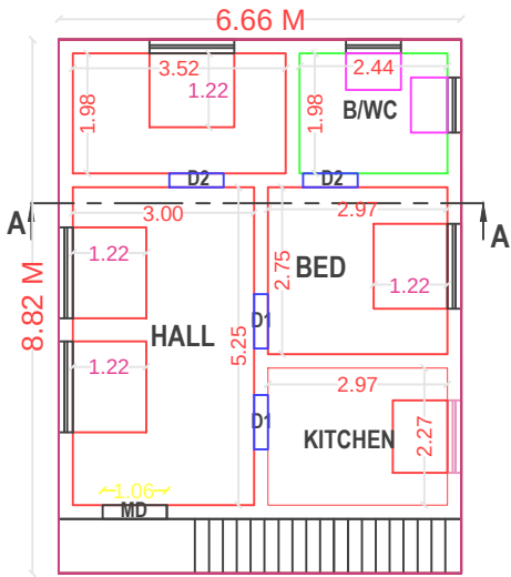
PLAN - GROUND FLOOR ( PROPOSED )
