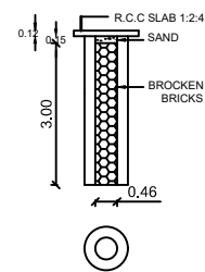
PERCOLATION PIT
