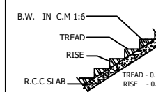
STAIR DETAILS
