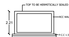
SECTION ON U.G.SUMP
