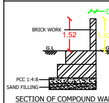
SECTION OF COMPOUND WALL
