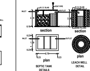
DETAILS OF FILTER BED & WELL
