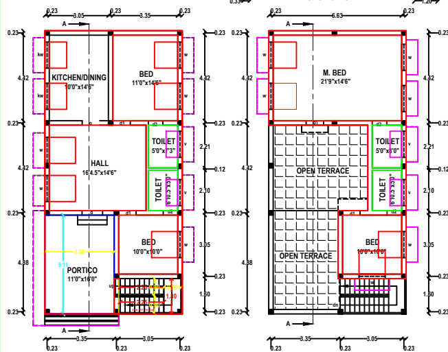
PLAN - RESIDENCE (EXISTING GROUND FLOOR)
