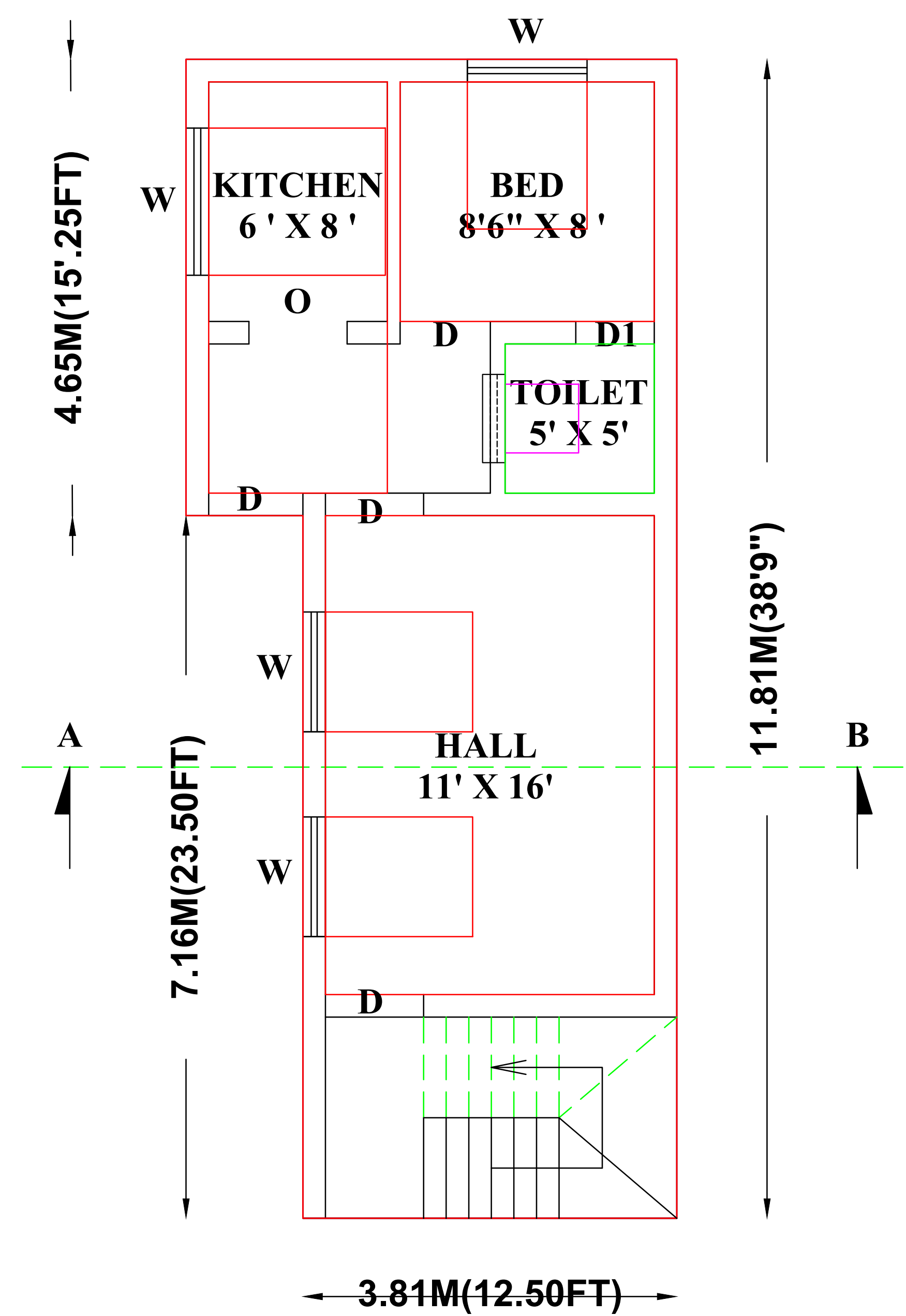
PLAN
