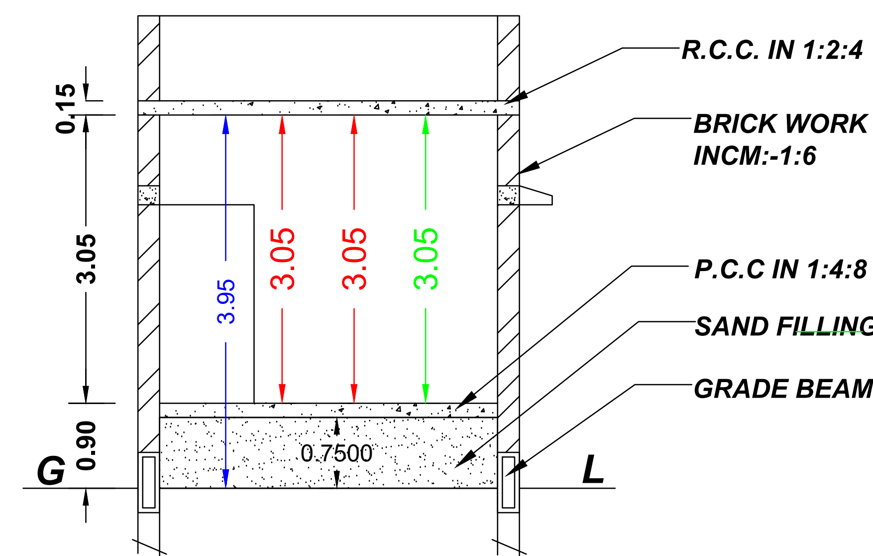
SECTION "AB"
