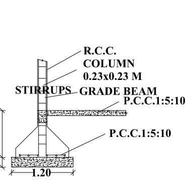
COLUMN DETAIL
