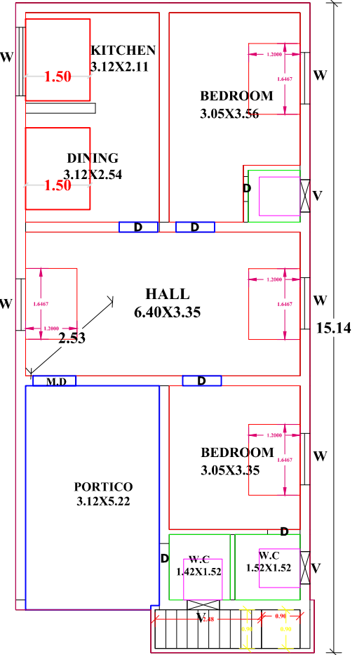
PLAN
