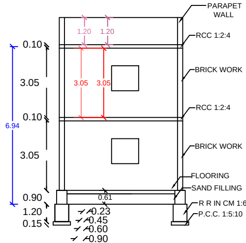
SECTION AB
