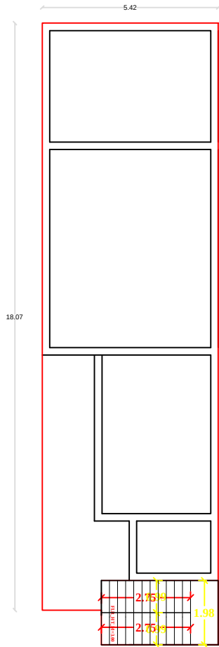
EXG.GROUND FLOOR PLAN
