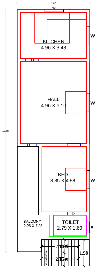
PRO.FIRST FLOOR PLAN
