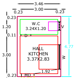
FLOOR PLAN
