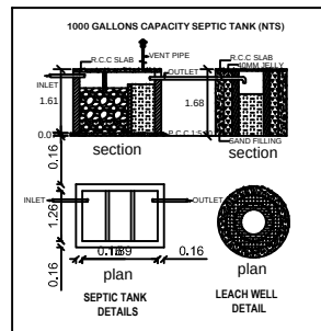
1000 GALLONS CAPACITY SEPTIC TANK (NTS)
