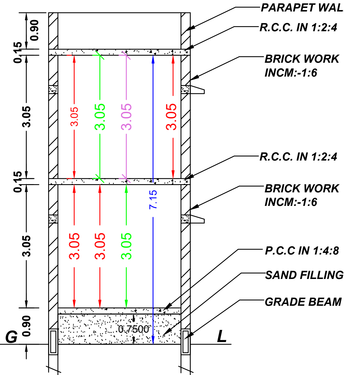
SECTION "AB"
