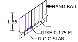
STAIRCASE
