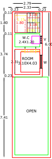
PRO FIRST FLOOR RESIDENTIAL PLAN
