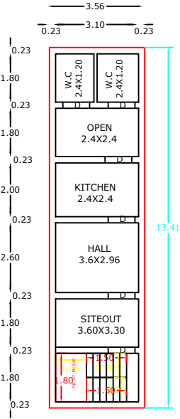
EXT GROUND FLOOR RESIDENTIAL PLAN
