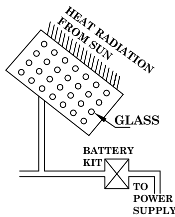
SOLAR SYSTEM
