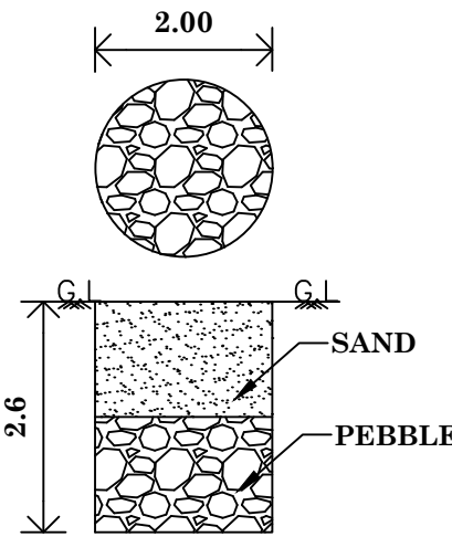
RAINWATER HARVESTING
