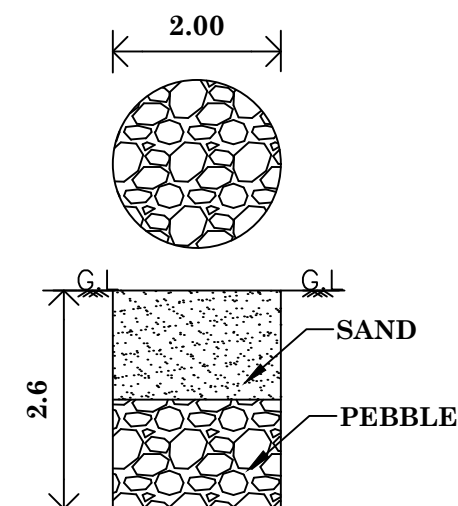
RAINWATER HARVESTING
