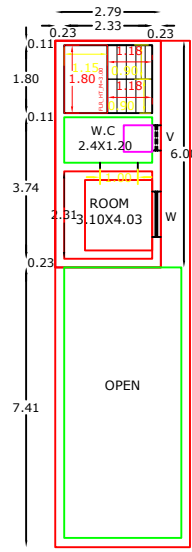
PRO FIRST FLOOR RESIDENTIAL PLAN
