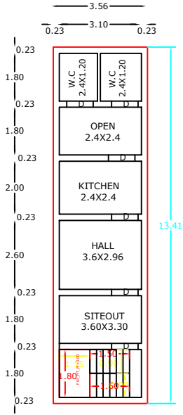
EXT GROUND FLOOR RESIDENTIAL PLAN
