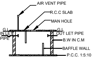
SECTION ON SEPTIC TANK
