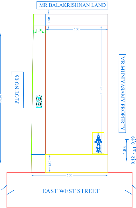
SITE PLAN
