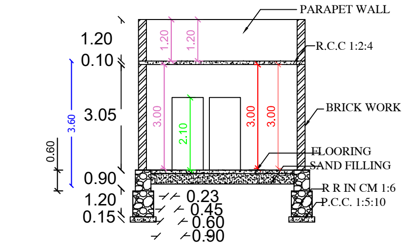
SECTION AB
