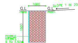
SECTION OF PEBBLE TRENCH
