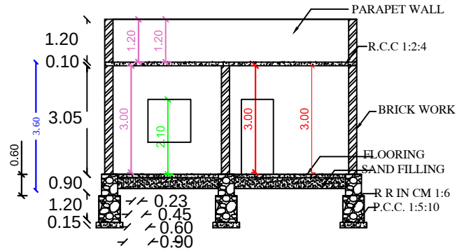
SECTION AB
