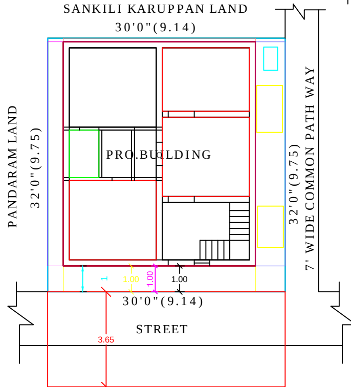
SITE PLAN
