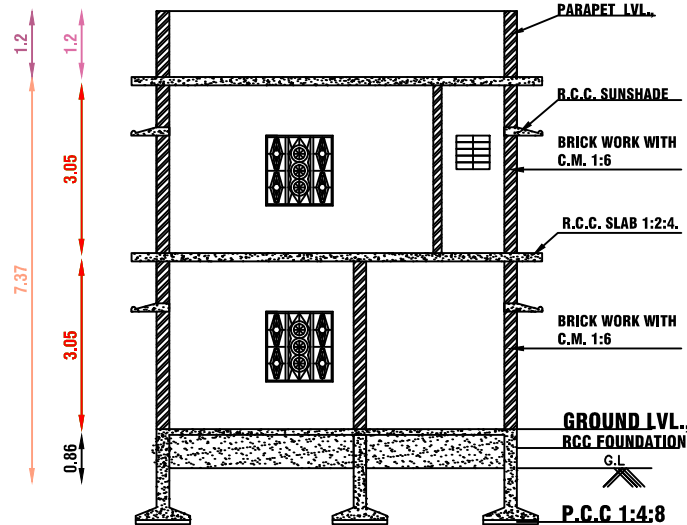
SECTION ON A-A & A'-A'
