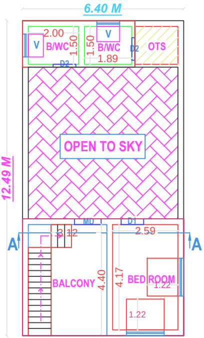
PLAN - FIRST FLOOR ( PROPOSED )
