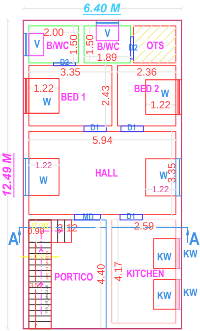
PLAN - GROUND FLOOR ( PROPOSED )
