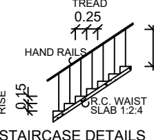
STAIRCASE DETAILS
