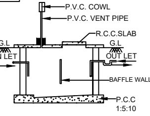
SEC. OF SEPTIC TANK
