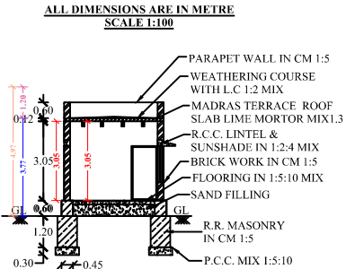
SECTION OF "AB"
