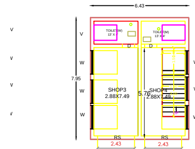
PROPOSED F.FLOOR
