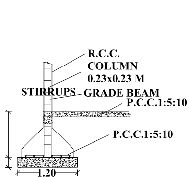
COLUMN DETAIL
