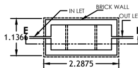
PLAN PLAN OF SEPTIC TANK
