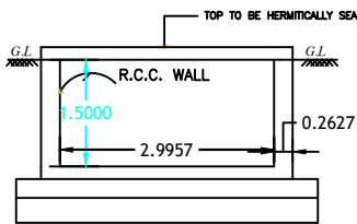
RWH SECTION
