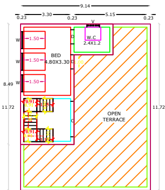
FIRST FLOOR RESIDENTIAL PLAN
