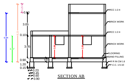
SECTION AB
