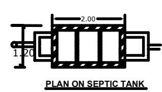
PLAN ON SEPTIC TANK
