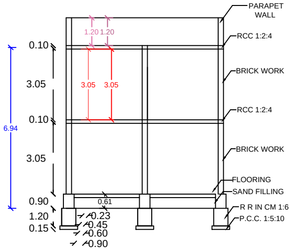
SECTION AB
