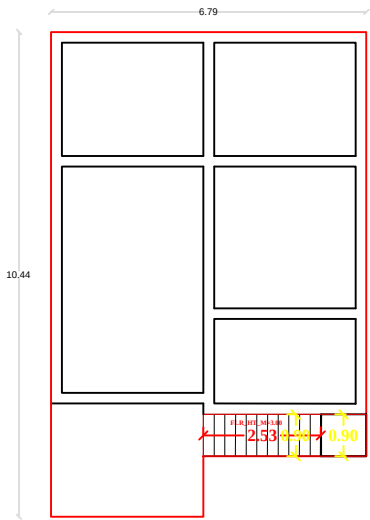
EXG GROUND FLOOR PLAN
