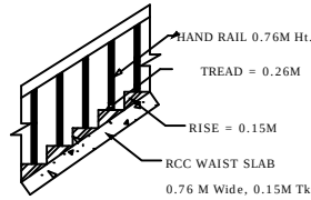
STAIRCASE DETAILS
