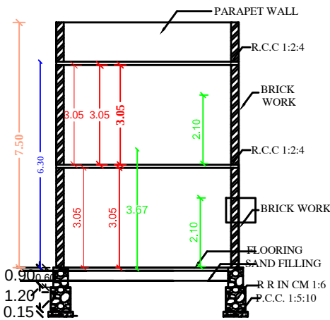
SECTION AB
