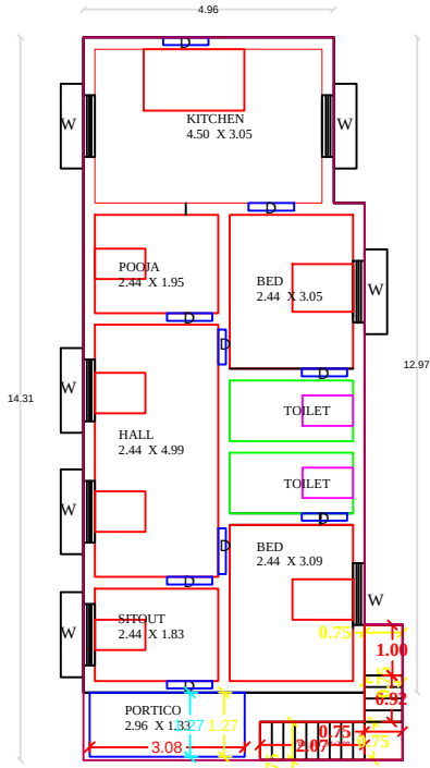
EXG.GROUND FLOOR PLAN
