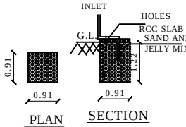
RAIN WATER COLLECTING TANK
