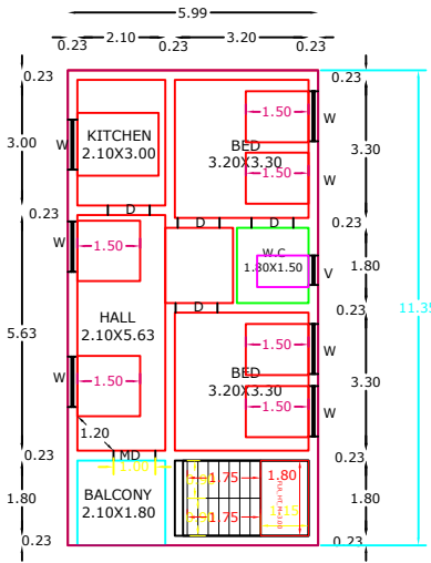
PRO FIRST FLOOR RESIDENTIAL PLAN
