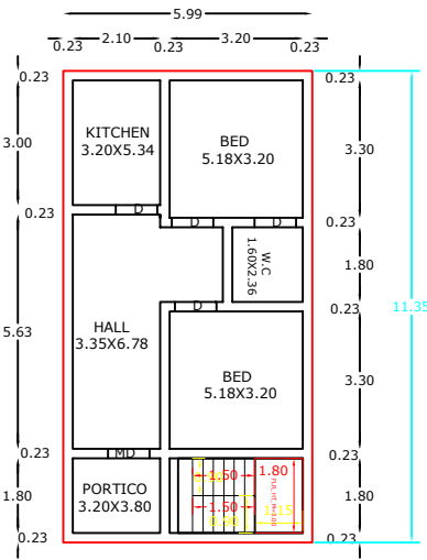
EXT GROUND FLOOR RESIDENTIAL PLAN
