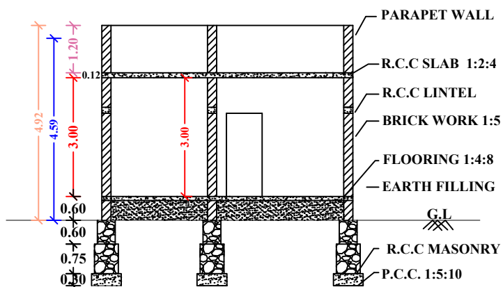
"SECTION "AB"
