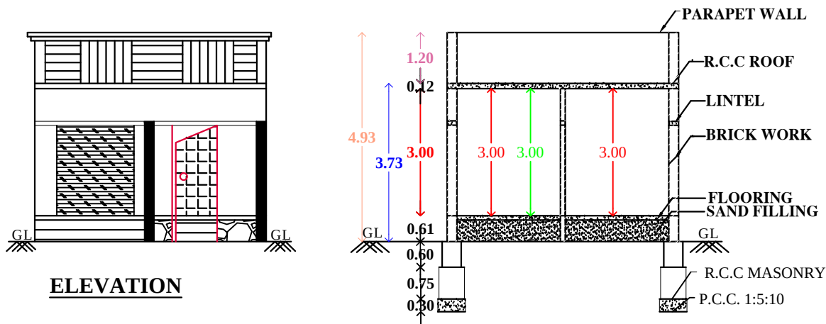
"SECTION "AB"
