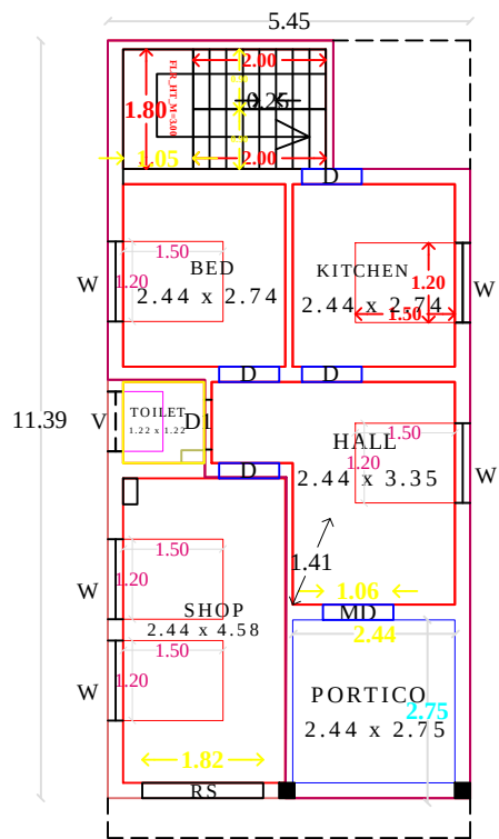
PLAN
