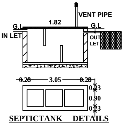
SEPTICTANK DETAILS
