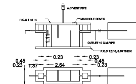
SEPTIC TANK &amp; TRENCH
