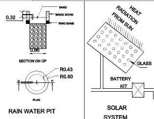
RAIN WATER PIT SOLAR SYSTEM
