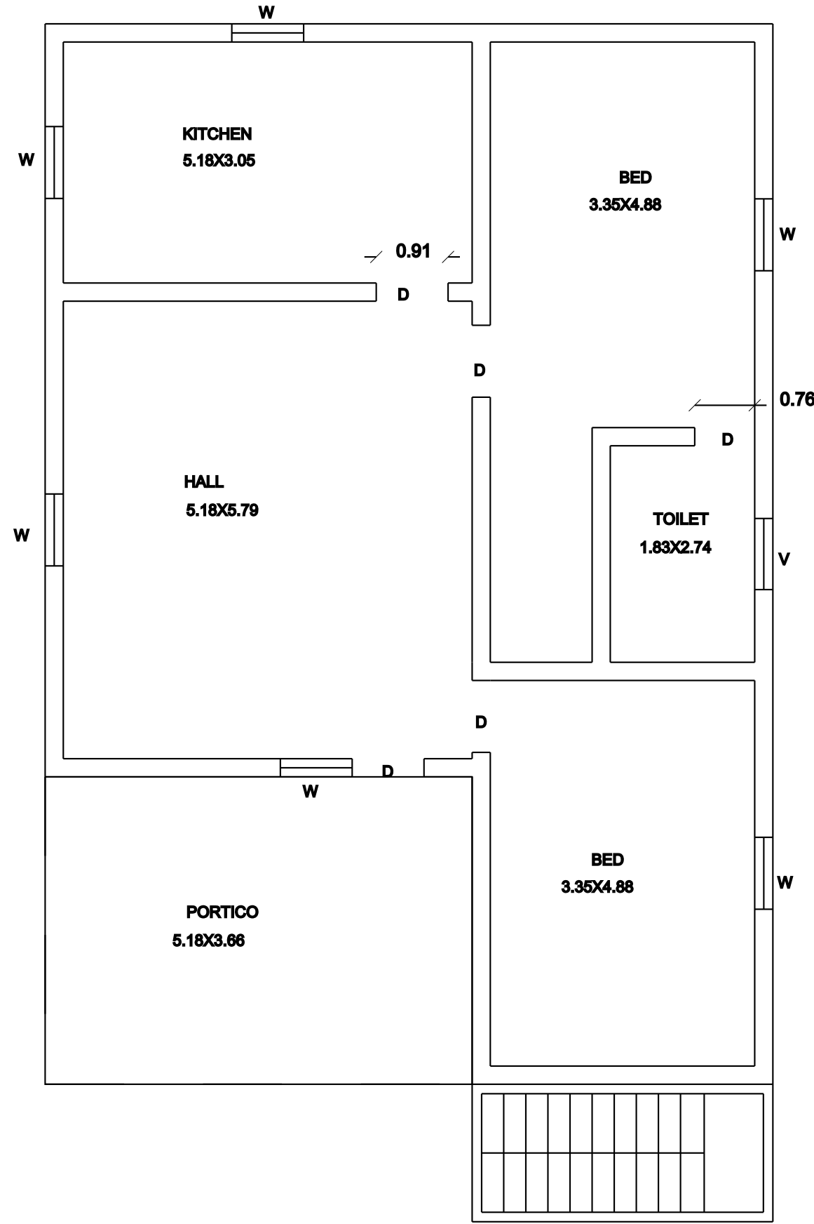
PLAN - GROUND FLOOR
