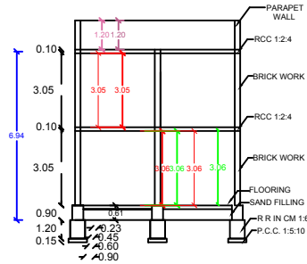
SECTION AB
