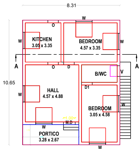
PLAN
