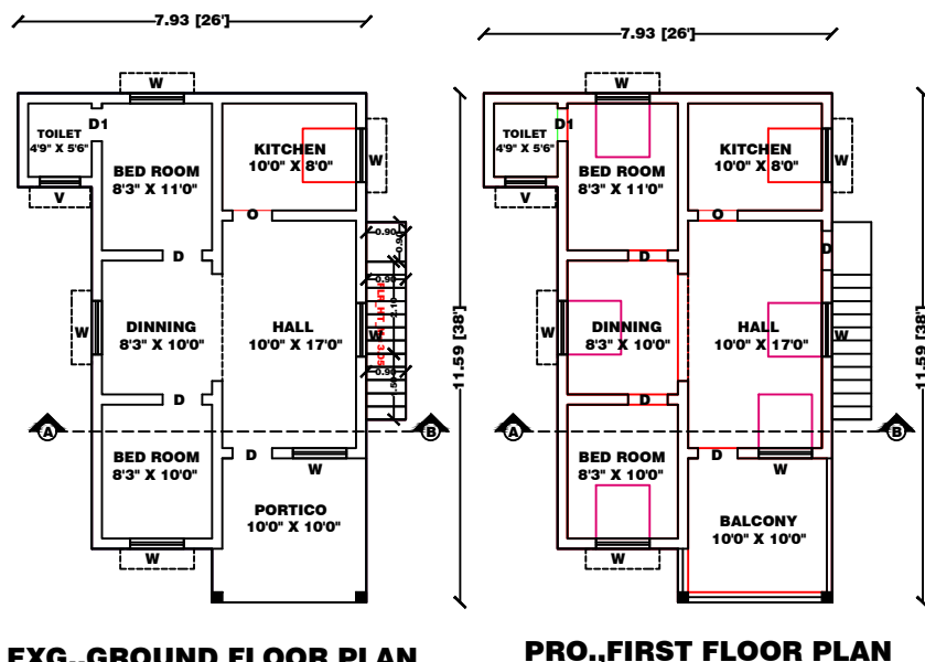
EXG.,GROUND FLOOR PLAN
