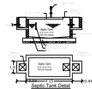
Septic Tank Detail
