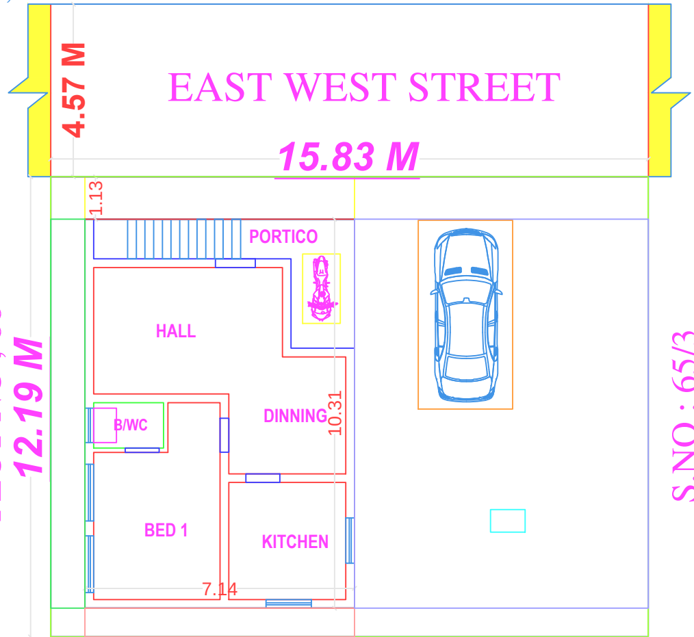
PLOT NO : 86 SITE PLAN SCALE:- 1:100
