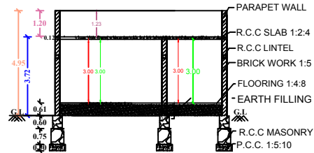
"SECTION "AB"
