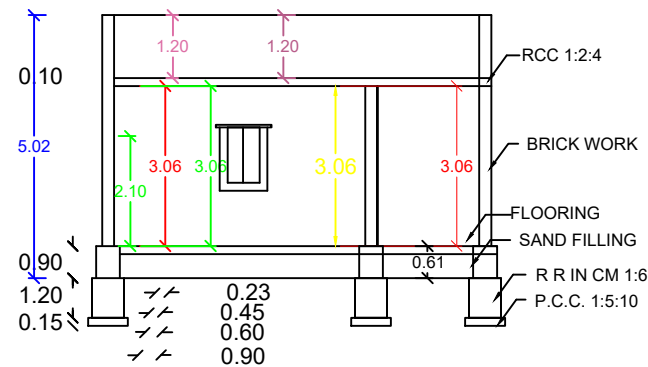
SECTION "AB"
