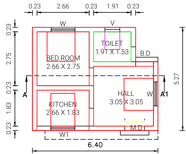
PLAN - GROUND FLOOR (PROPOSED)
