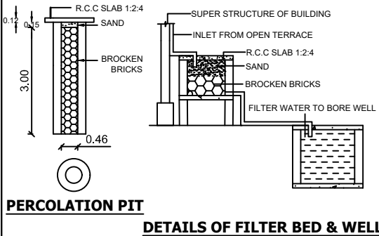
DETAILS OF FILTER BED & WELL
