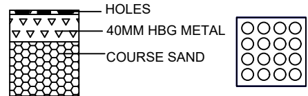
RAIN WATER COLLECTING TANK
