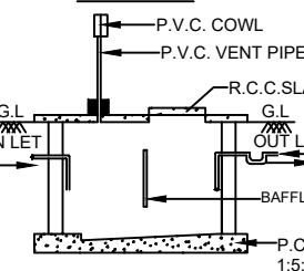
SEC. OF SEPTIC TANK
