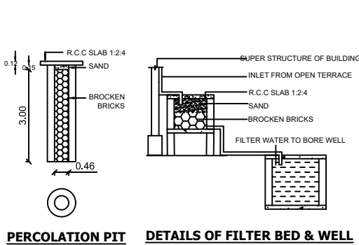
PERCOLATION PIT DETAILS OF FILTER BED & WELL
