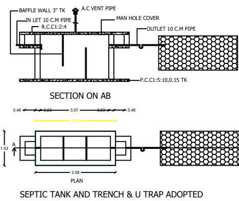
SEPTIC TANK AND TRENCH & U TRAP ADOPTED
