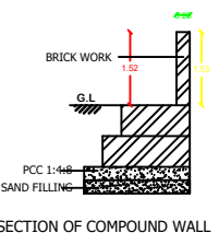
SECTION OF COMPOUND WALL
