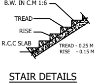
STAIR DETAILS
