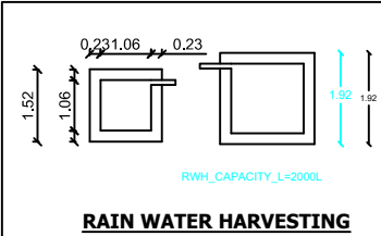
RAIN WATER HARVESTING
