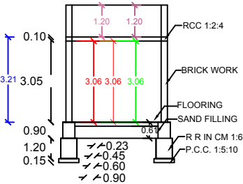
SECTION AB
