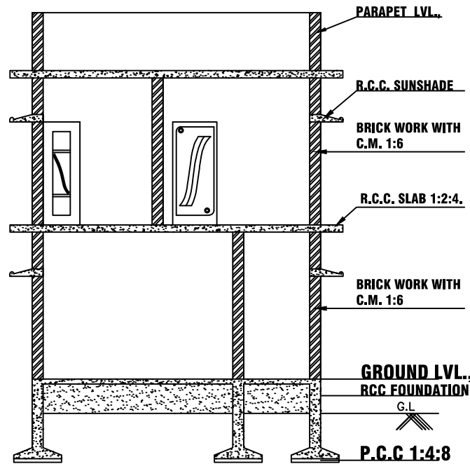
SECTION ON A-A & A'-A'
