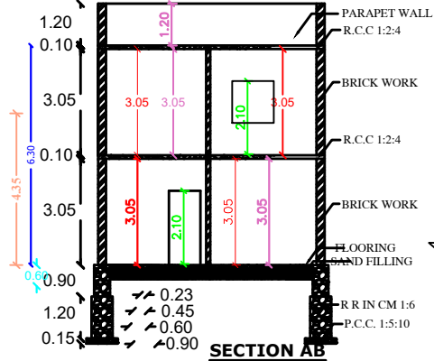
SECTION AB
