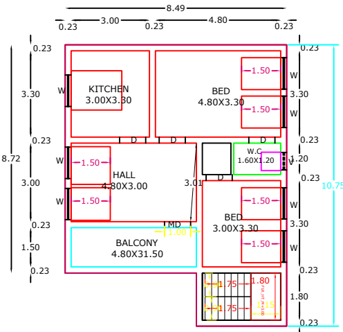
PRO FIRST FLOOR RESIDENTIAL PLAN
