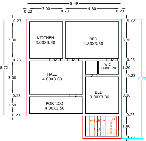
EXT GROUND FLOOR RESIDENTIAL PLAN
